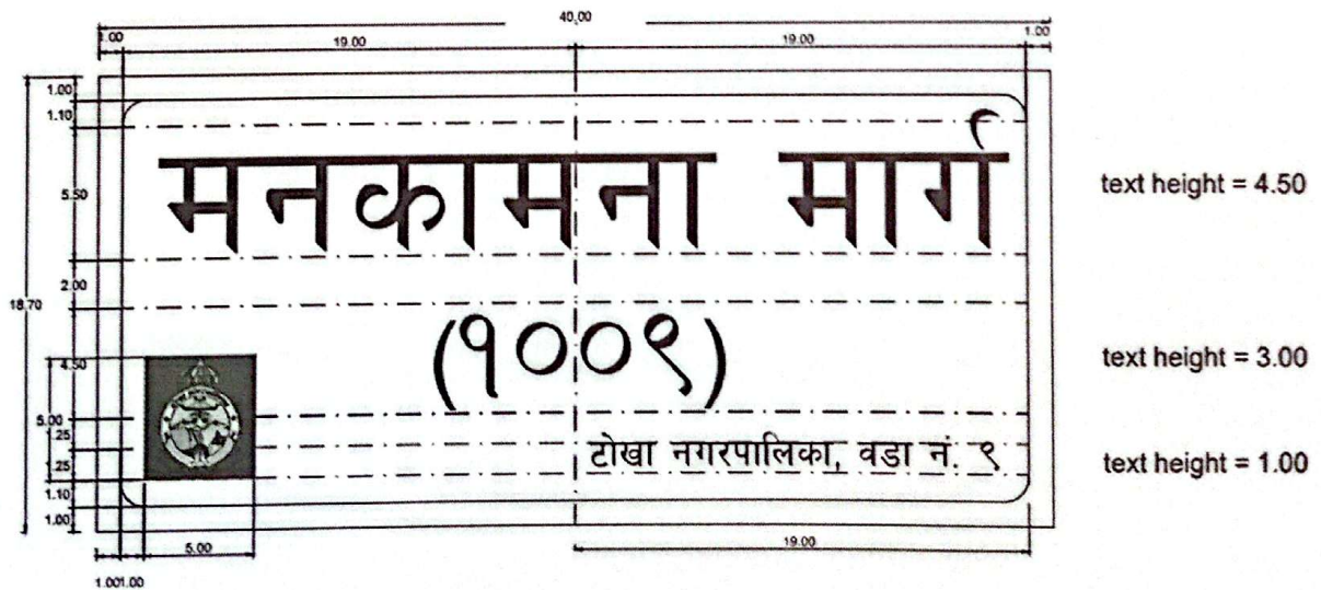
Fig. 4: Street Signage Board for Minor and Subsidiary Roads — Nepali Only
