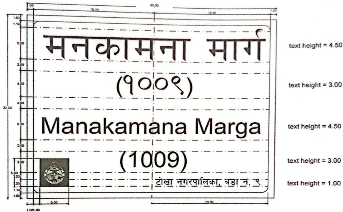
Fig. 5: Street Signage Board for Major or Minor Road Junctions — Nepali and English
