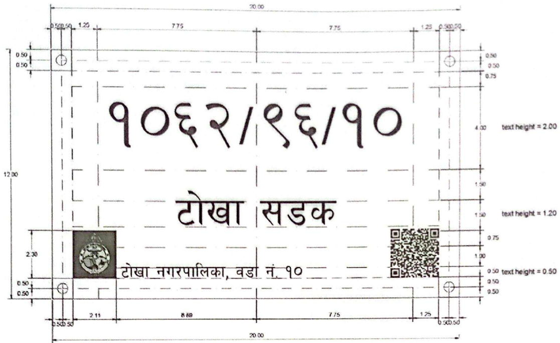
Fig. 3: Sample House Address Plate — Two Levels Off from a Major or Minor Road (Double Slash)
