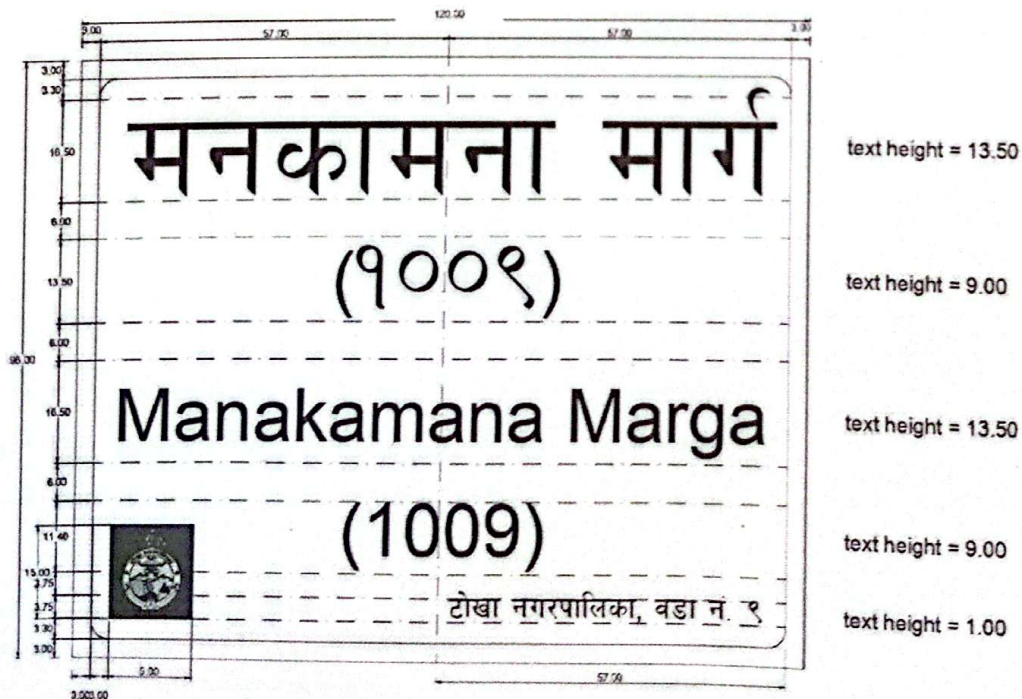
Fig. 6: Street Signage Board for Major Road Junctions — Nepali and English with Double-Pole Mounting
